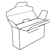
7624 4-3/16" W x 7-3/8" H 2-1/6" Capacity [1] Fold Over Flap w. Tuck Tab [Side 'Wings'] [1] Wrap Around Flap w. Tuck Tab
