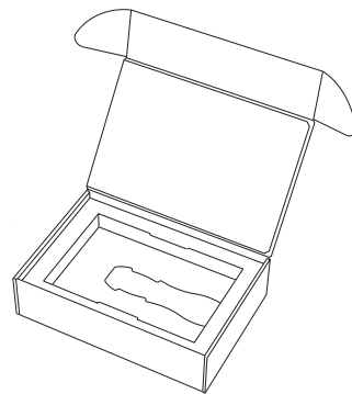
M0526 9-1/2" x 6-1/2" x 2-1/2" 7-1/2" x 5" x 1" Well Custom Die Cut to Hold Tool
