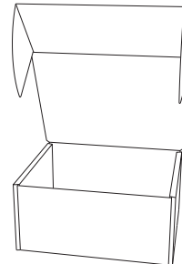
M00336D 4-3/4" W x 4" H x 2-3/8" D Econo Style, 2 Side Rollover with Cover Flaps
