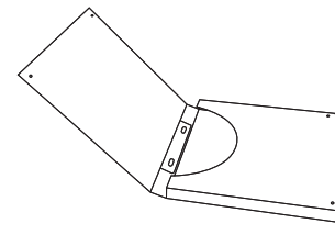
7578 11-1/2" W x 11-9/16" H, 1" Capacity Full Super Constructed Flap Tuck End w. Lock Tabs Designed w. Plastic Handle [Optional]
